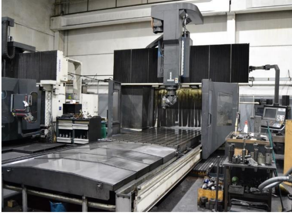
Fresadora puente NICOLAS CORREA FP 40-40S Mesa: 4500x2000mm. Recorridos: 4000x3100x1000mm Control HEIDENHAIN iTNC 530 y volante electrónico NICOLAS CORREA FP 40-40S bridge milling machine Table: 4500x2000mm. Travels: 4000x3100x1000mm HEIDENHAIN iTNC 530 control and electronic wheel
